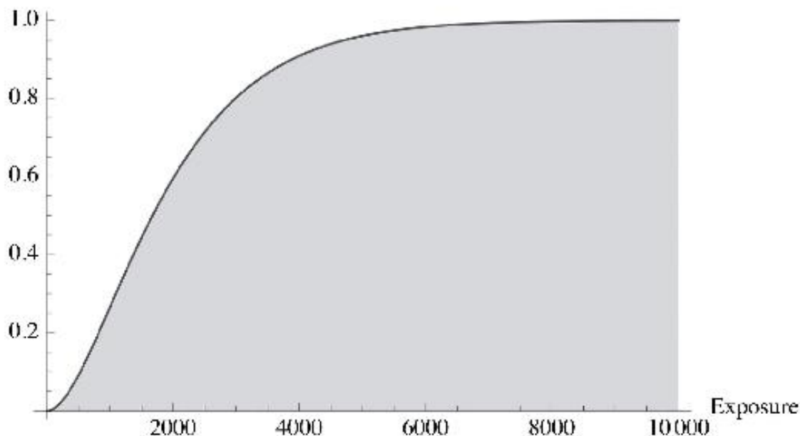
Probability of Ruin
